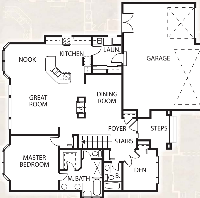
PLAN 1769 RANCHER 58'0 Width x 59'0 Depth
